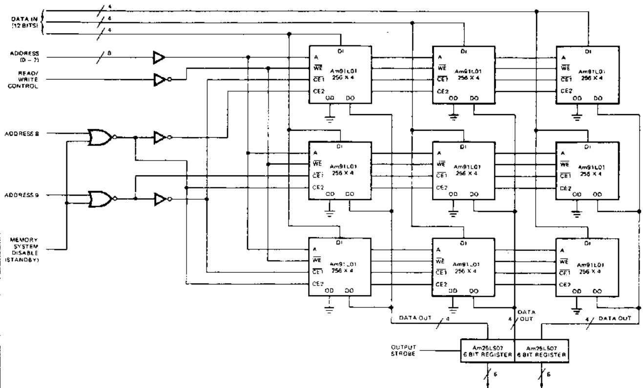
Figure 1. Memory System 768 Words by 12 Bits Per Word
