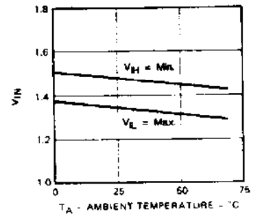
Typical VIH Limits Versus Ambient Temperature
