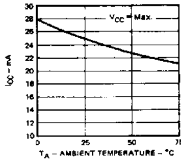
Typical Power Supply Current Versus Ambient Temperature
