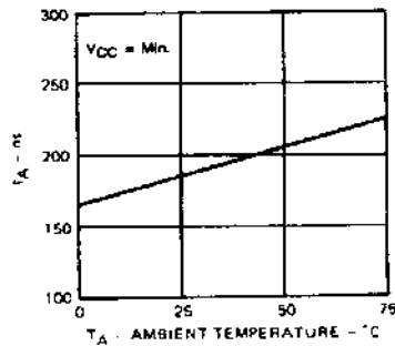
Typical tA Versus Ambient Temperature
