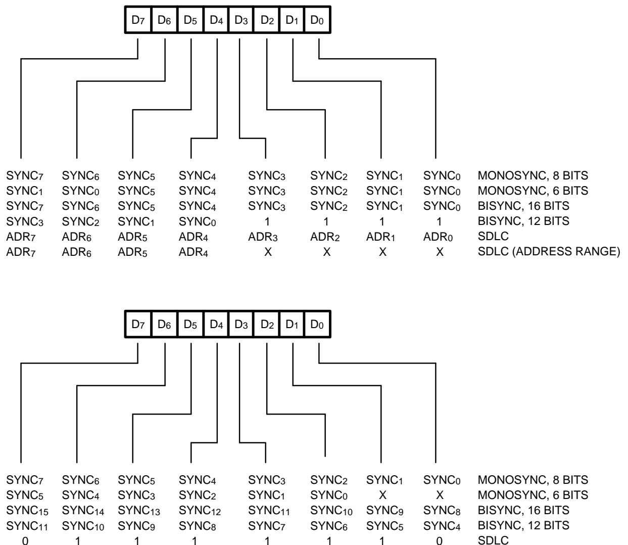
Figure 4-23. SYNC Character Programming
