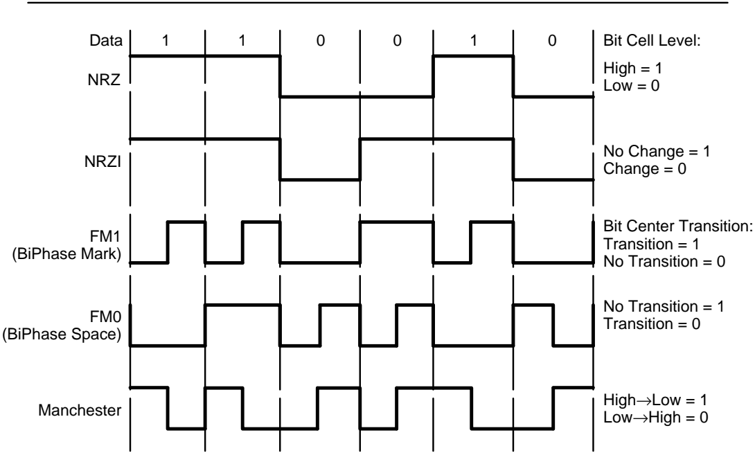
Figure 5–4. Data Encoding
