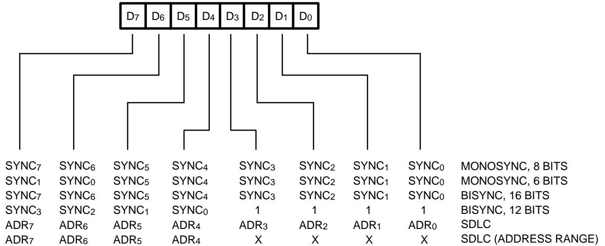
Figure 6–7. Write Register 6
