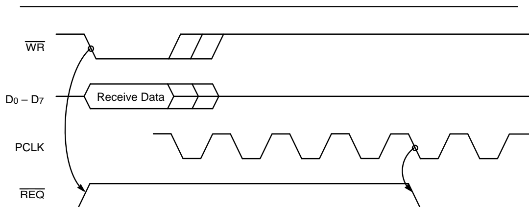
Figure 3–11. \overline{\text{DTR/REQ}} Deactivation
