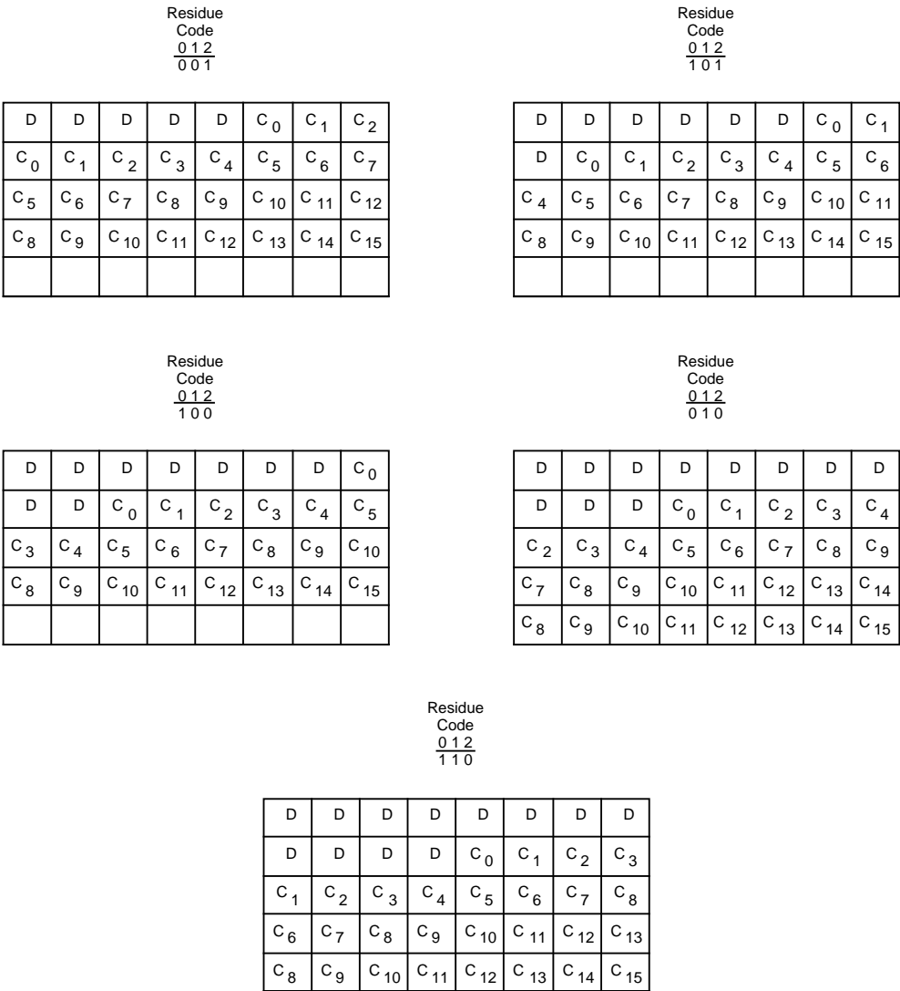
Figure 4–15. Five Bits/Character
