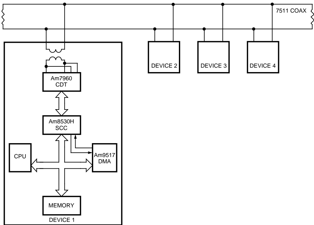
Figure 7-19. Bus Architecture
