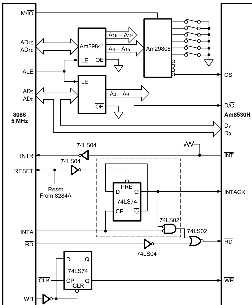
Figure 7-6. 8086—SCC Interface
