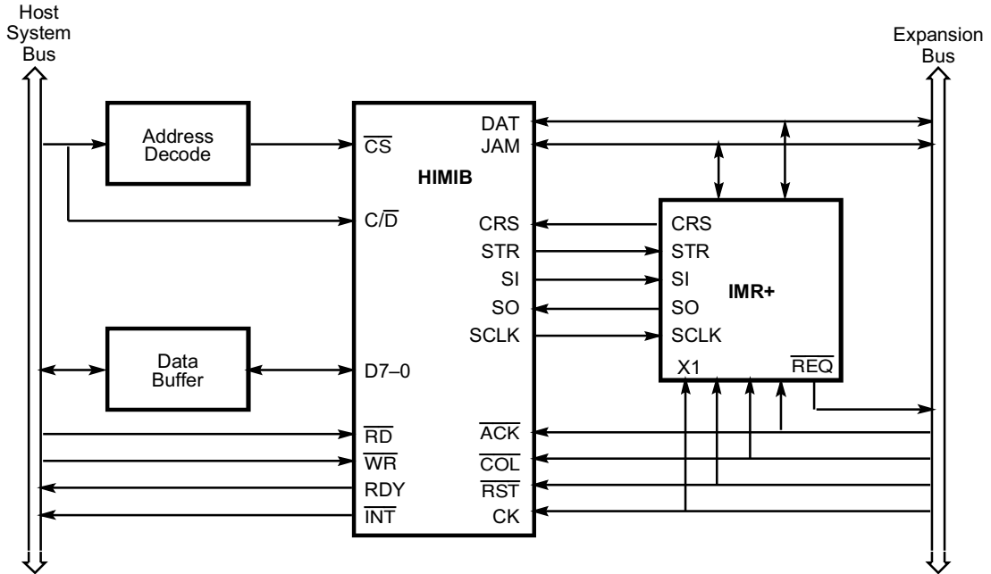
Figure 2. HIMIB Device Application Example
