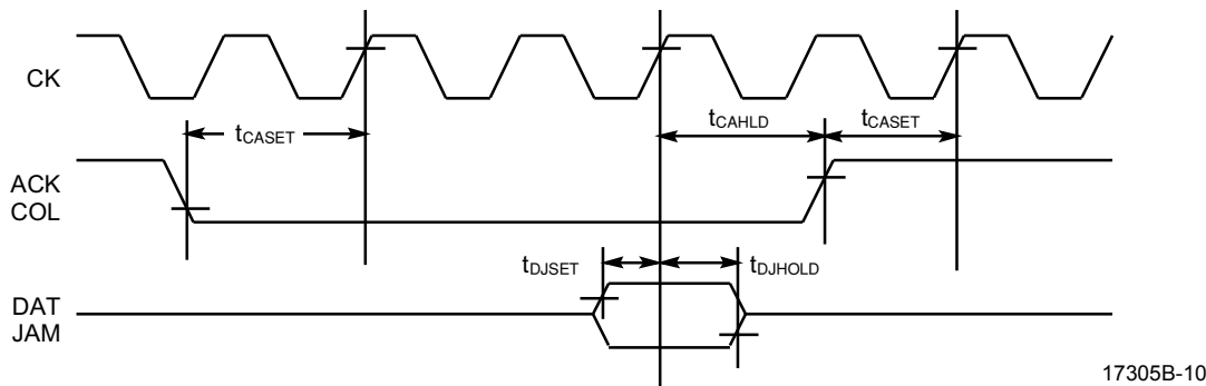
Expansion Port Timing
