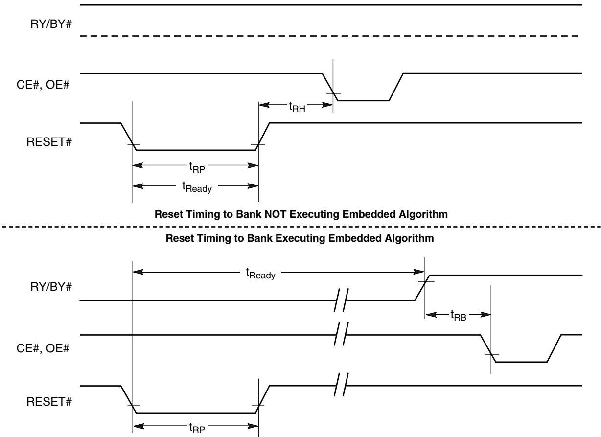
Figure 19. RESET# Timings
