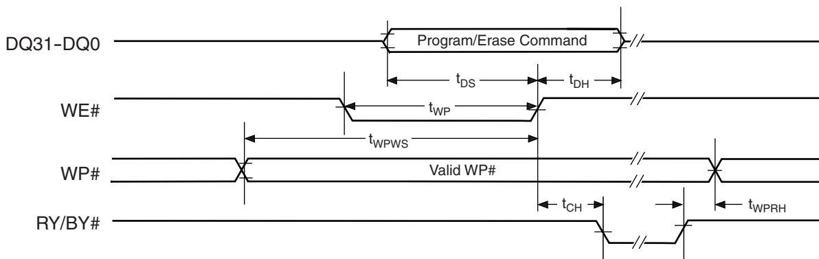
Figure 20. WP# Timing
