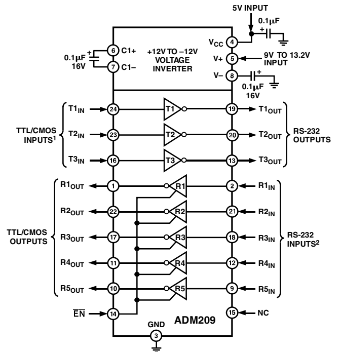
Figure 8. ADM209 Typical Operating Circuit
