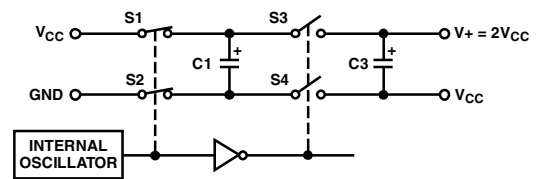
Figure 13. Charge-Pump Voltage Doubler
