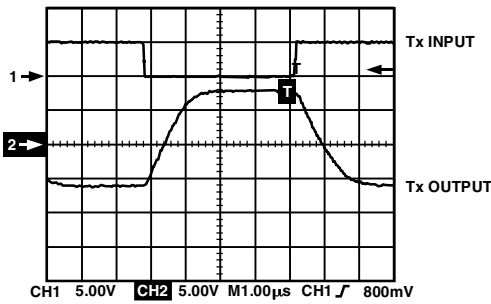
TPC 7. Transmitter Output Loaded Slew Rate
