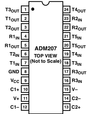
Figure 3. ADM207 DIP/SOIC/SSOP Pin Configuration
