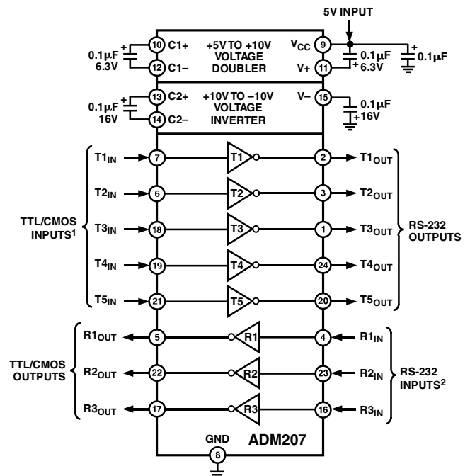
Figure 4. ADM207 Typical Operating Circuit
