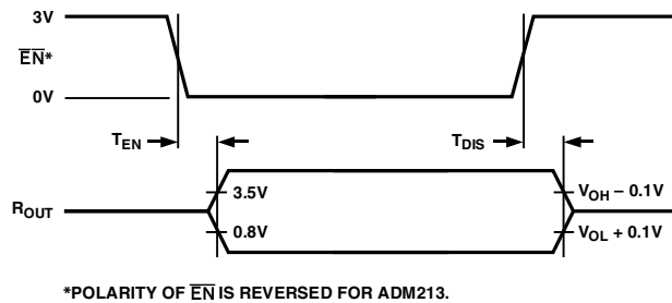
Figure 15. Enable Timing
