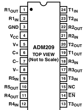
Figure 7. ADM209 DIP/SOIC/SSOP Pin Configuration
