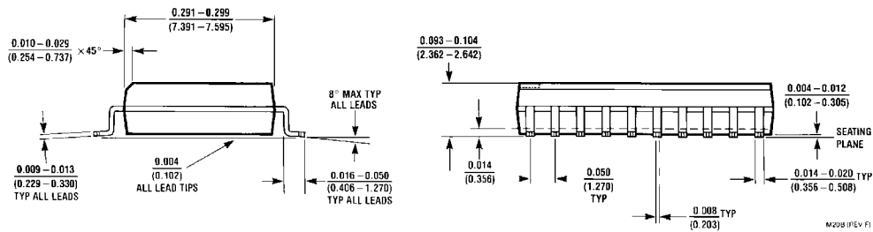
Order Number ADC10061CIWM NS Package Number M20B
