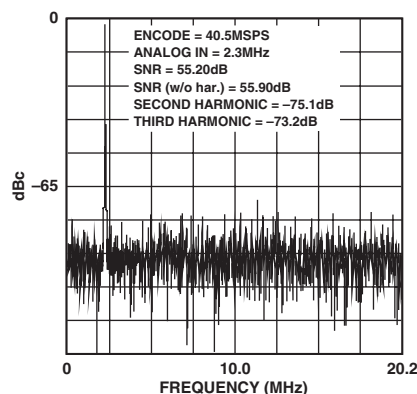
TPC 11. FFT Response
