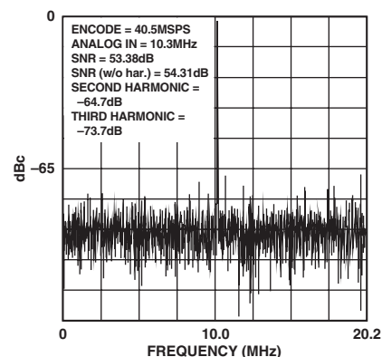
TPC 12. FFT Response
