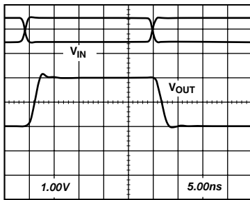
TPC 85. AD8130 Transient Response with +3 V Common-Mode Input
