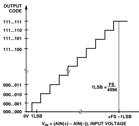
Figure 16. Unipolar Transfer Characteristic
