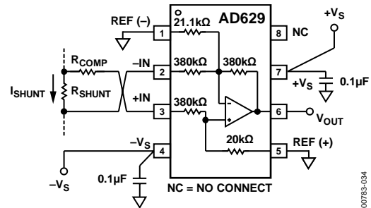
Figure 34. Compensating for Large Sense Resistors
