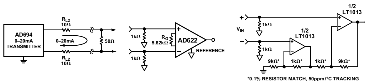
0–20 mA Current Loop with 50 \Omega Shunt Impedance
