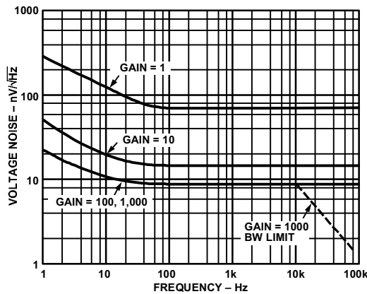
Figure 4. Voltage Noise Spectral Density vs. Frequency, (G = 1–1000)
