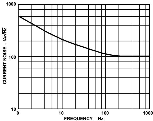
Figure 5. Current Noise Spectral Density vs. Frequency
