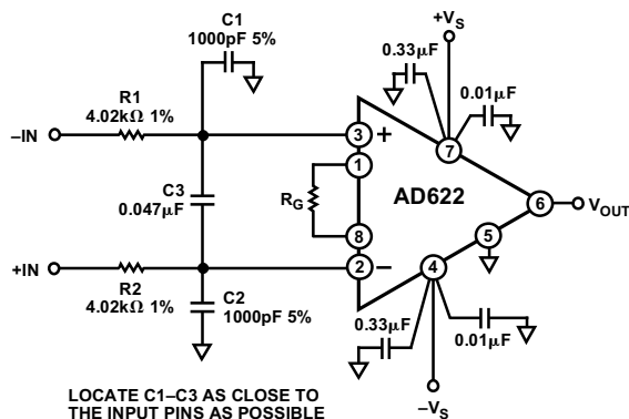
Figure 15. RFI Suppression Circuit for AD622 Series In-Amps
