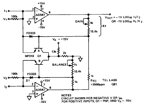
Figure 33. Log-Ratio Amplifier
