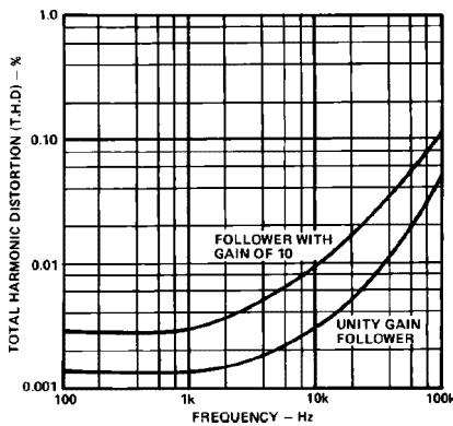
Figure 16. AD544 Total Harmonic Distortion vs. Frequency
