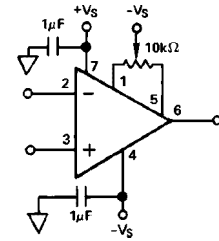
Figure 20. Standard Null Circuit
