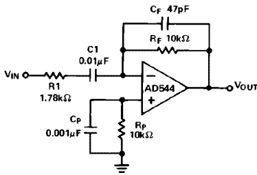
Figure 34. Differentiator
