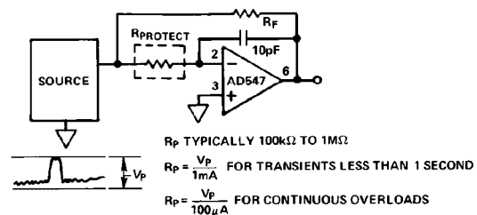
Figure 30. Input Protection
