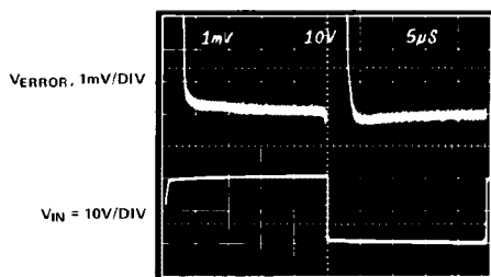
Figure 26. Settling Characteristic Detail-AD544
