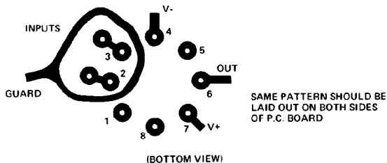
Figure 29. Board Layout for Guarding Inputs
