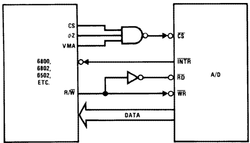
6800 Interface
