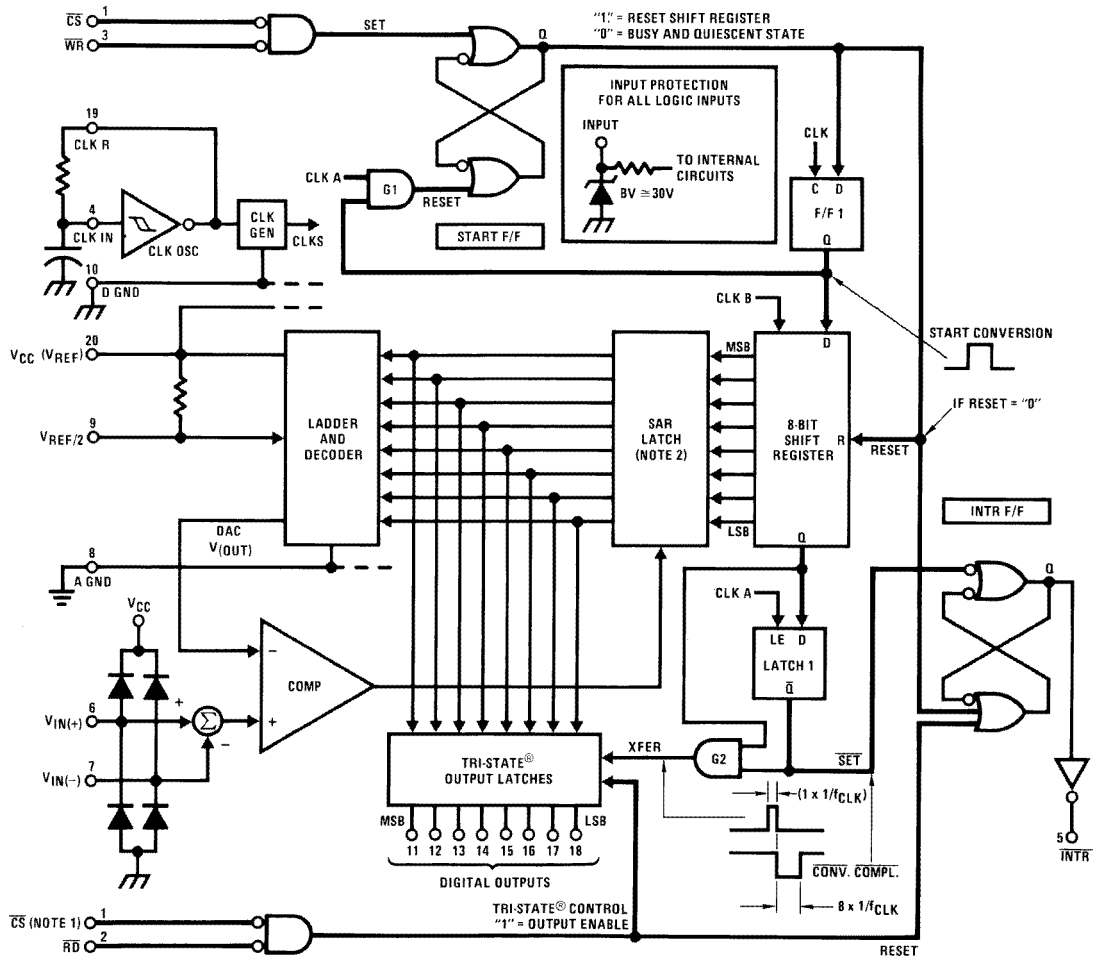
FIGURE 4. Block Diagram
