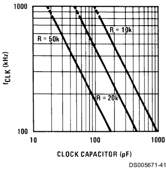
fCLK vs. Clock Capacitor
