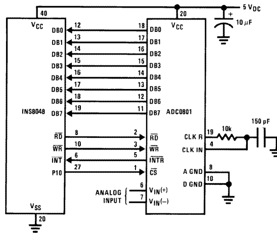
FIGURE 13. INS8048 Interface
