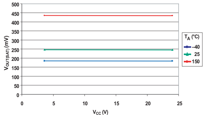
Output Voltage (On) versus Supply Voltage
