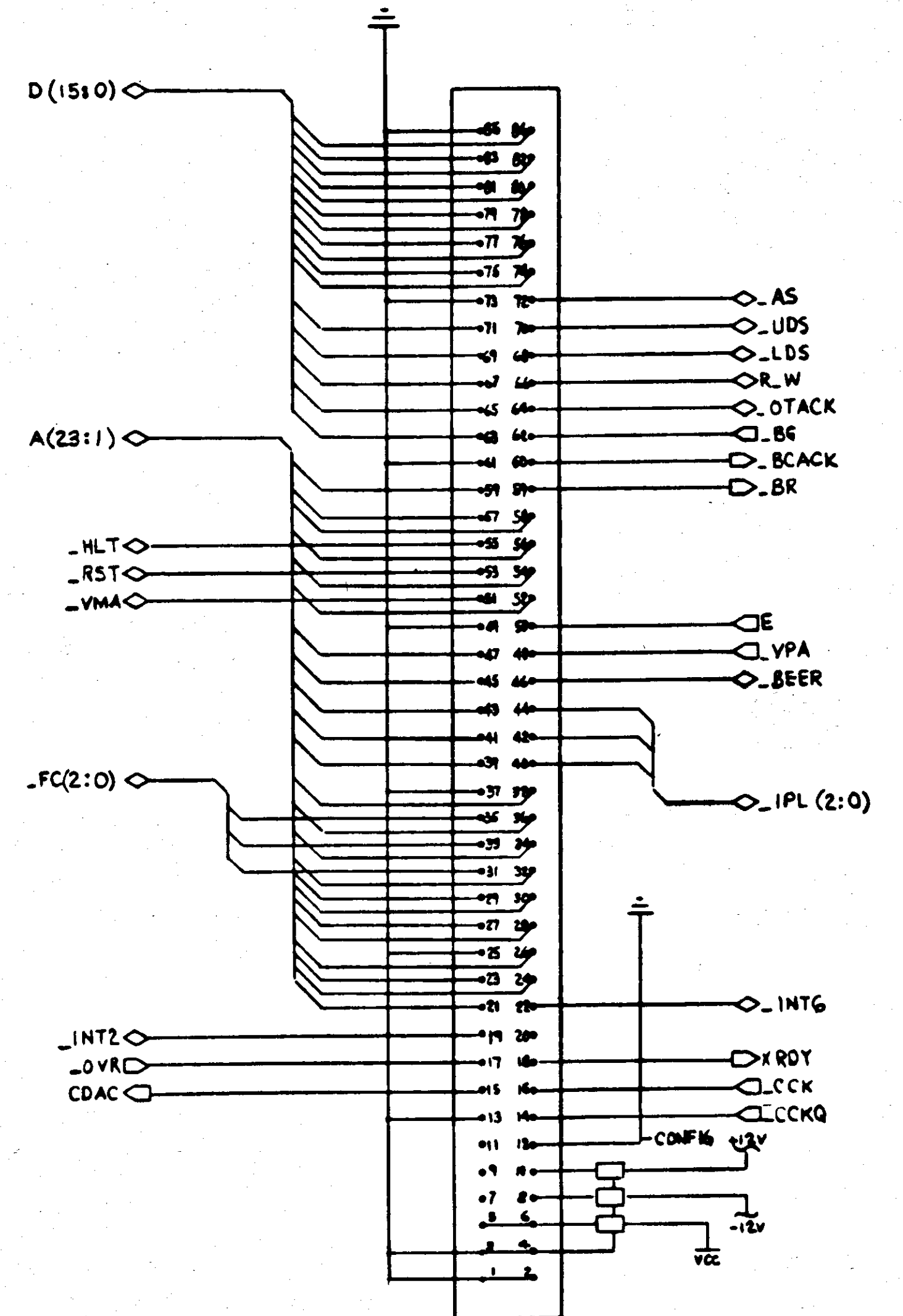
EXPANSION SCHEMATIC
