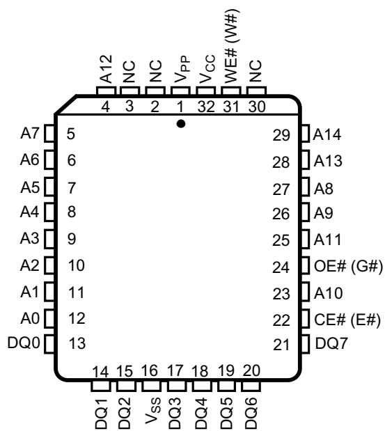
PLCC
