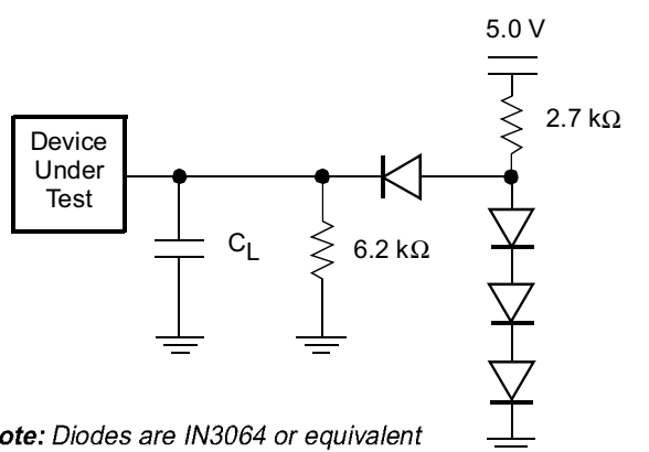
Figure 6. Test Setup
