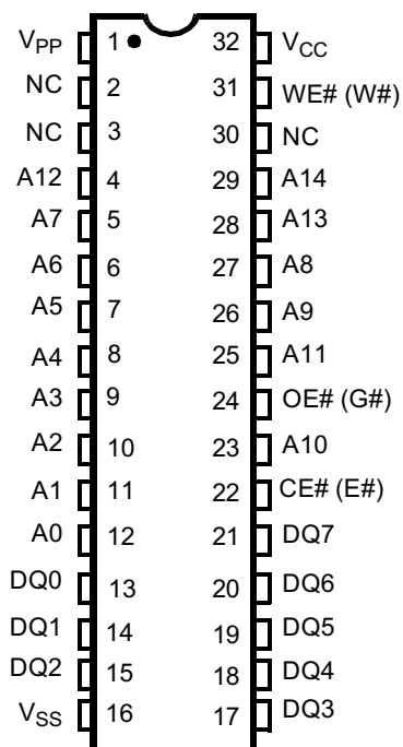
PDIP
