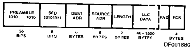
Figure 9-2. IEEE 802.3 MAC Frame Format
