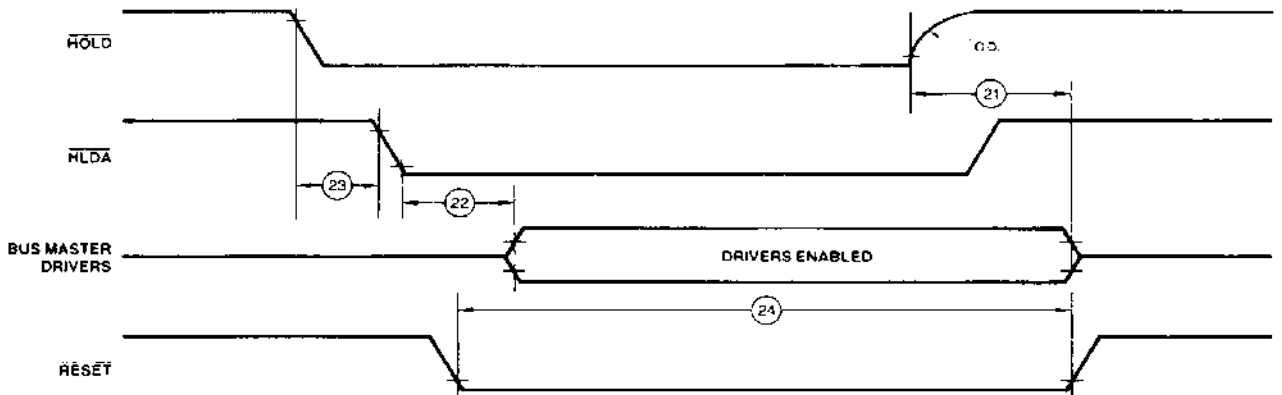
Figure 6. Bus Acquisition Timing
