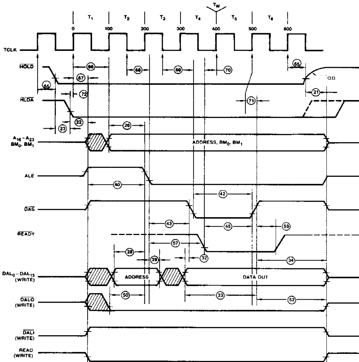
Figure 5-2. Bus Master Write Timing (Single DMA Cycle)
