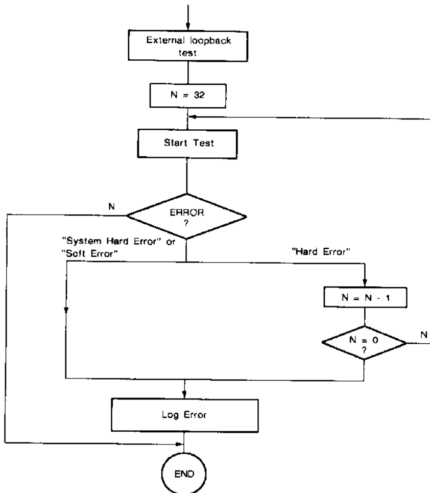
Figure 9. External Loopback Test Flow Chart
