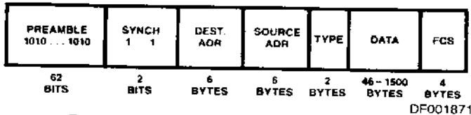
Figure 9-1. Ethernet Frame Format
