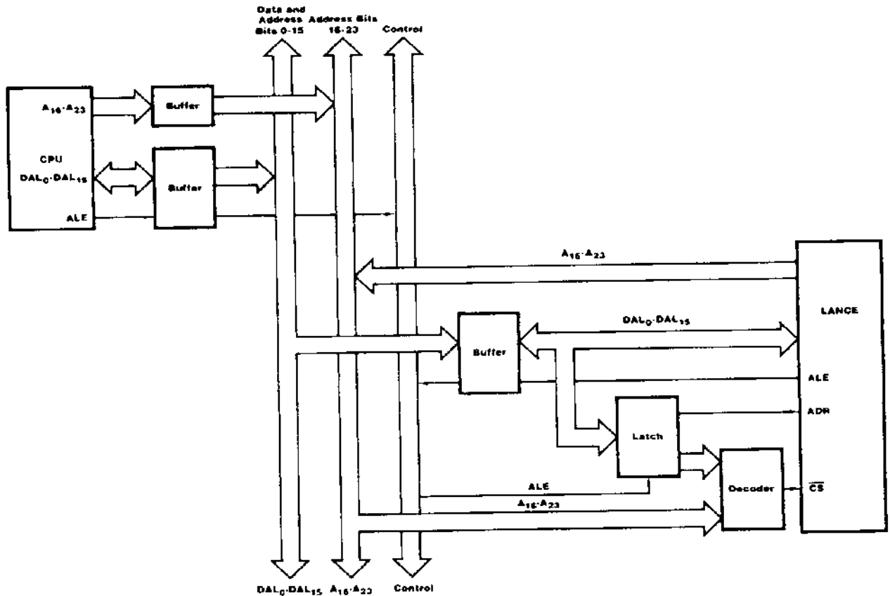
Figure 1-1. LANCE/CPU Interfacing — Multiplexed Bus
