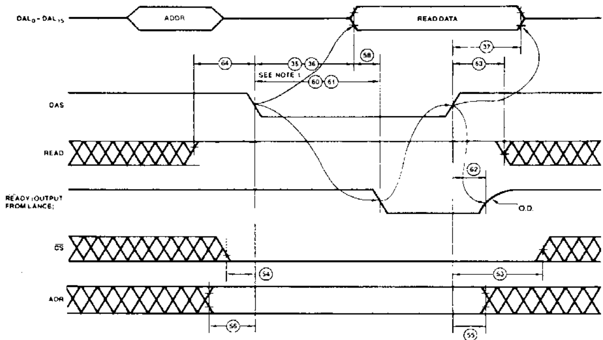
Figure 3. Bus Slave Read Timing
