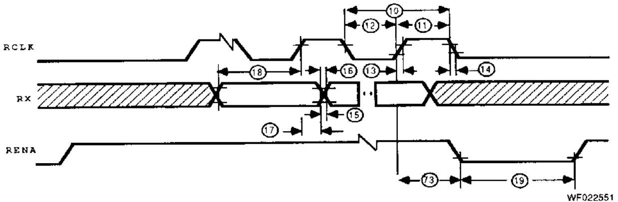
Serial Link Timing (Receive)
