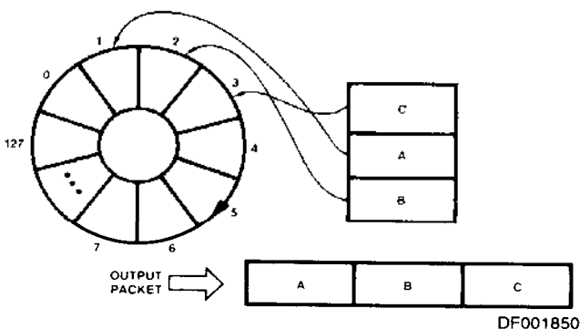
Figure 8-1. Data Chaining (Transmit)
