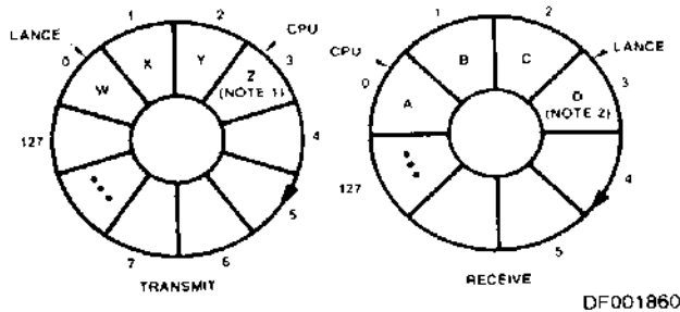
Figure 8-2. Buffer Management Descriptor Rings
