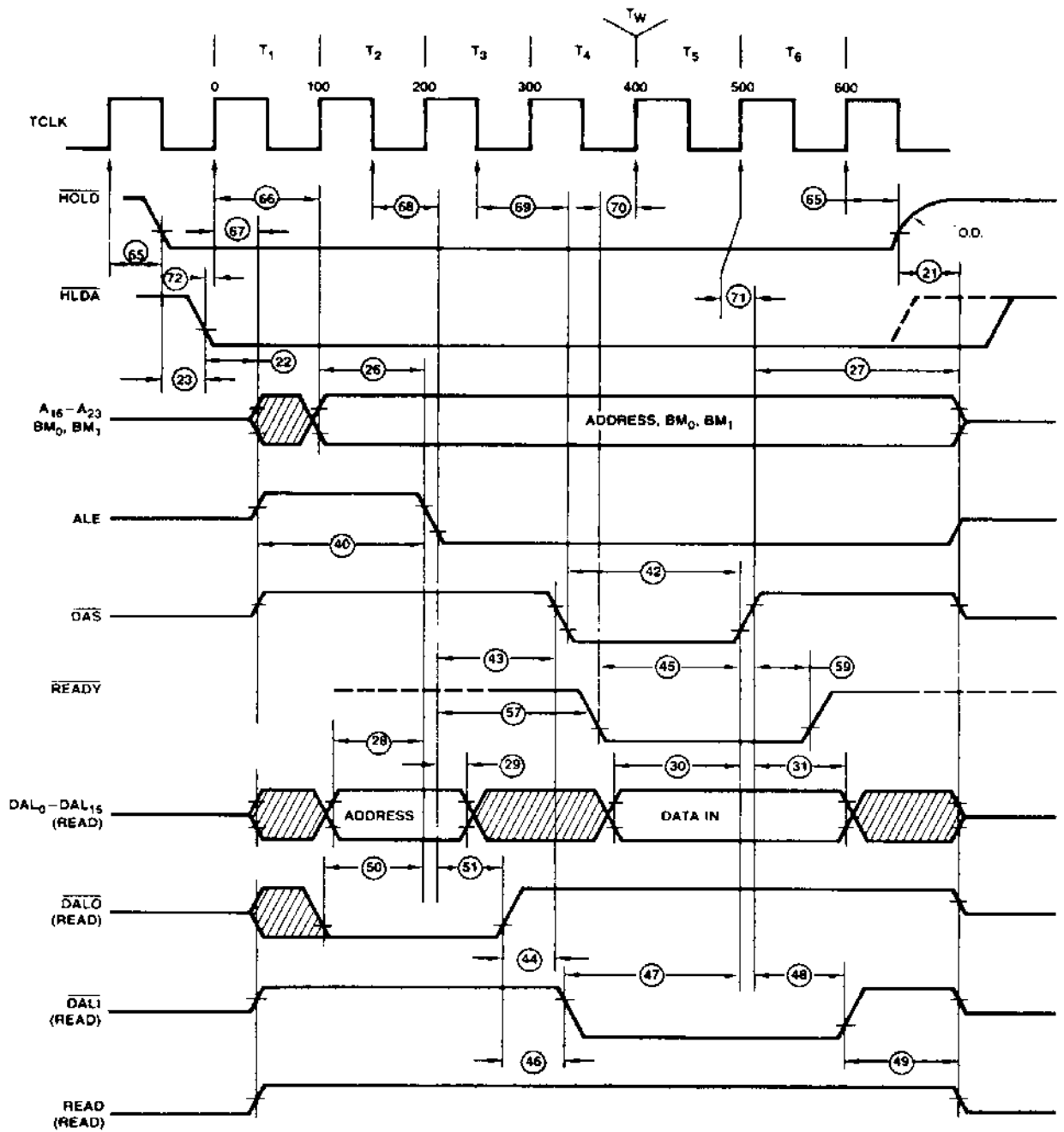
Figure 5-1. Bus Master Read Timing (Single DMA Cycle)
