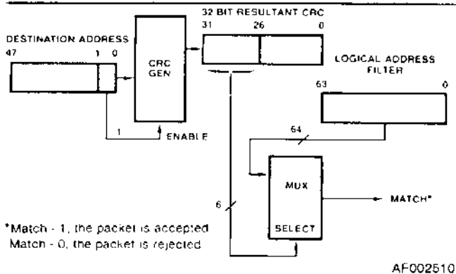
Figure 7. Logical Address Filter Operation
