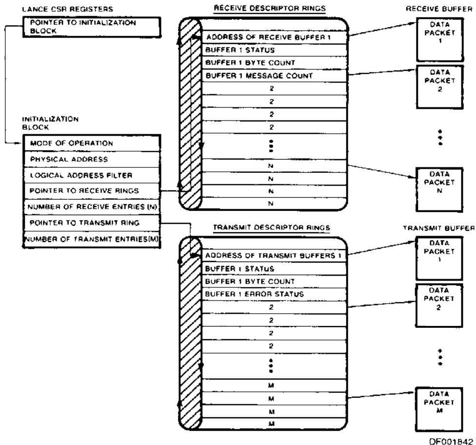
Figure 2-2. LANCE Memory Management
