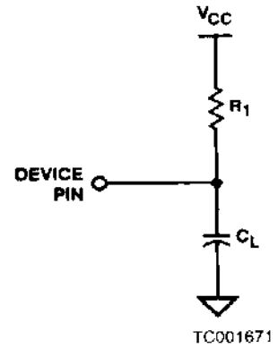
B. Open-Drain Outputs ( \overline{\text{INTR}} , \overline{\text{HOLD/BUSRQ}} , \overline{\text{READY}} )
