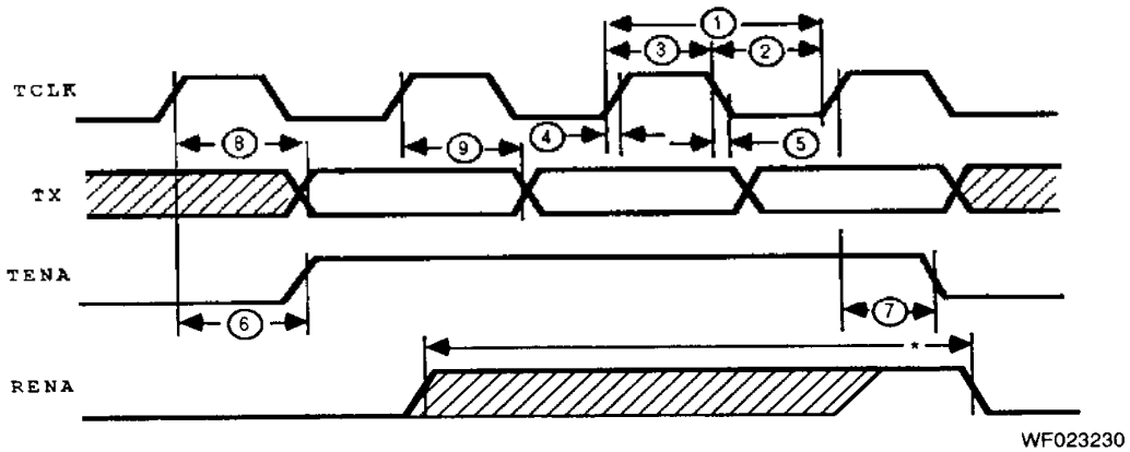
Serial Link Timing (Transmit)
