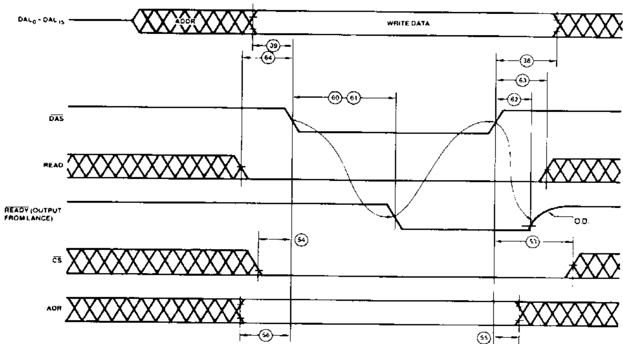
Figure 4. Bus Slave Write Timing
