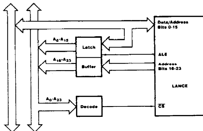
Figure 1-2. LANCE/CPU Interfacing — Demultiplexed Bus
