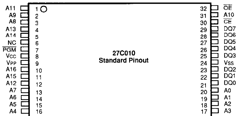
Am27C010 128K x 8 EPROM in 32 Lead TSOP
