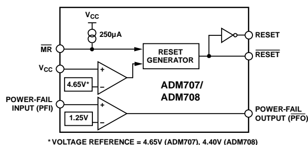
Figure 2. ADM707/ADM708
