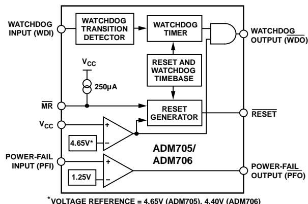
Figure 1. ADM705/ADM706
