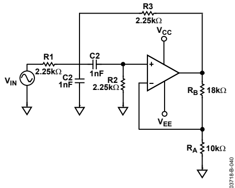
Figure 38. Band-Pass KRC Filter
