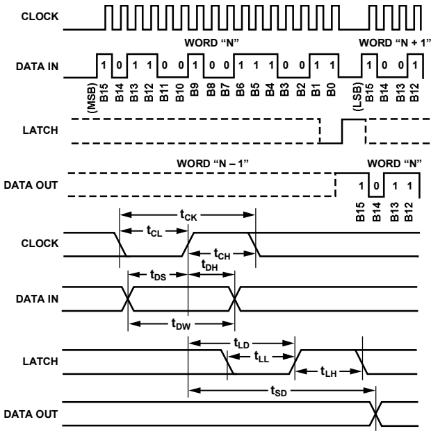
Figure 3. Timing Diagram for 3-Wire Interface
