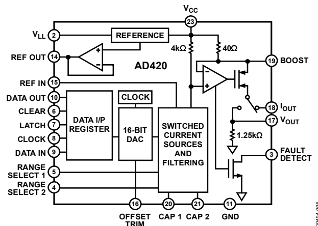
Figure 5. Functional Block Diagram
