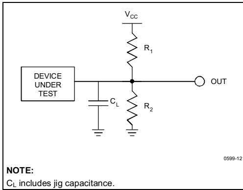
Figure 13. Test Configuration
