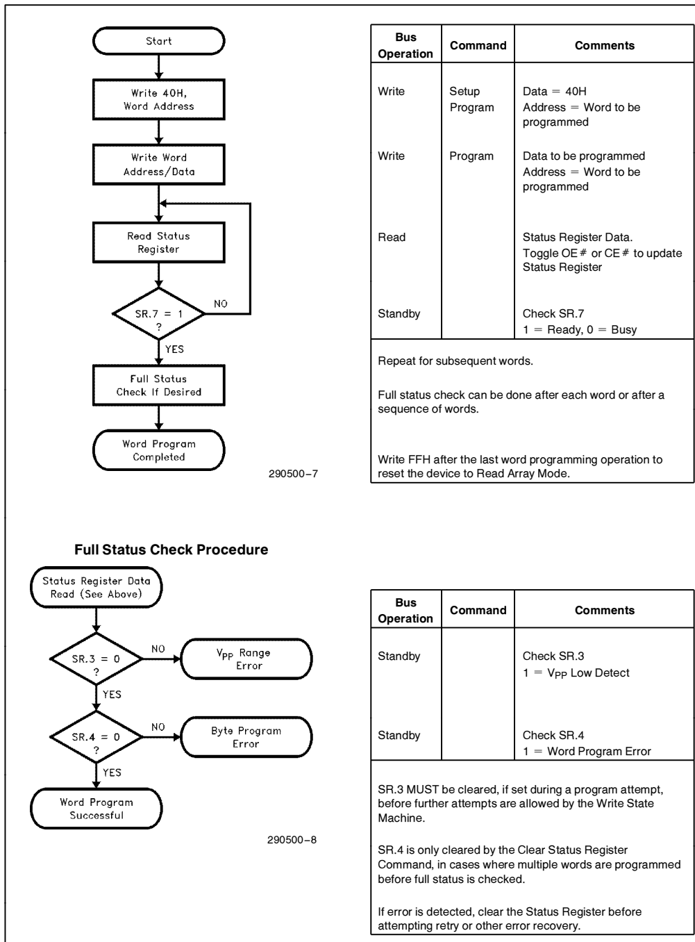
Figure 7. Automated Word Programming Flowchart
