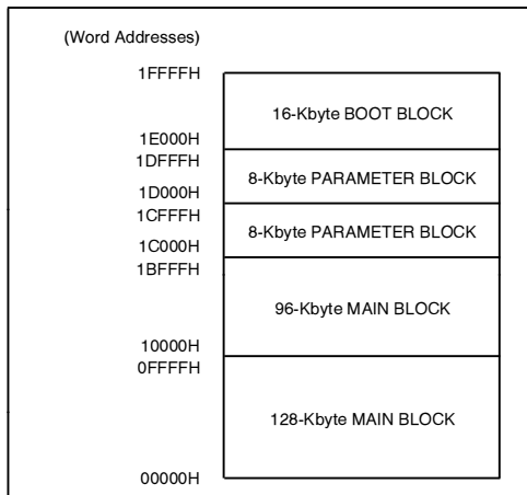
Figure 5. A28F200BX-T Memory Map
