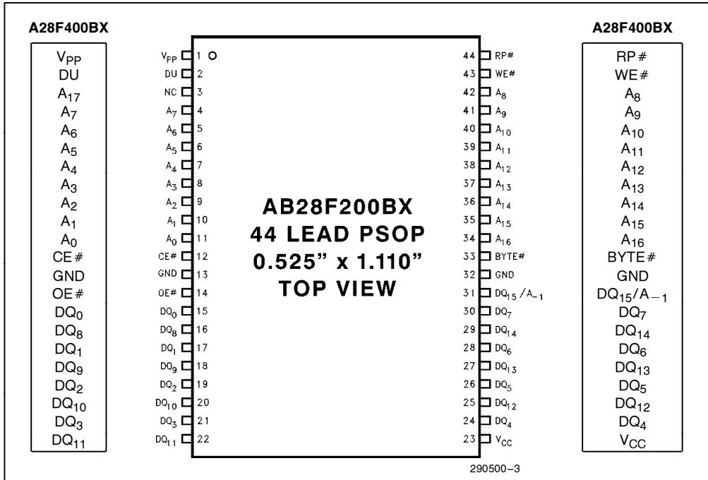
Figure 2. PSOP Lead Configuration
