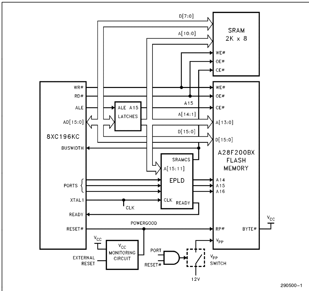
Figure 1. A28F200BX Interface to 8XC196KC
