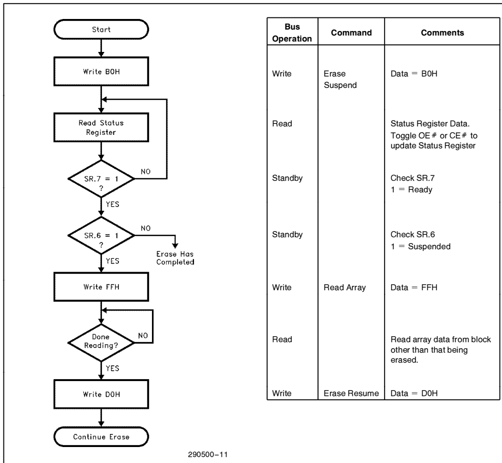
Figure 9. Erase Suspend/Resume Flowchart
