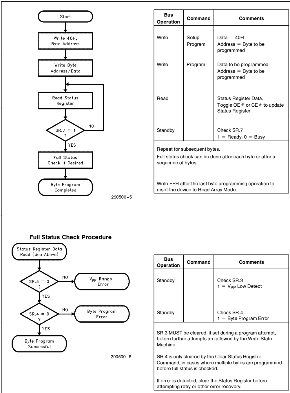
Figure 6. Automated Byte Programming Flowchart
