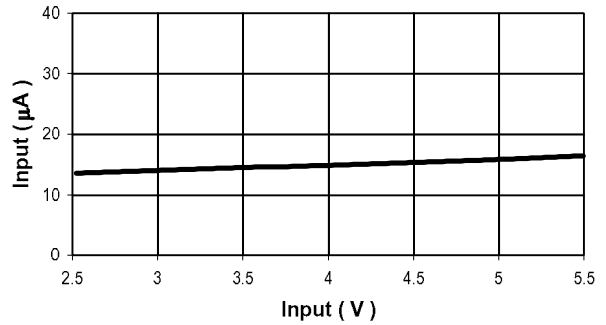
Quiescent Current
