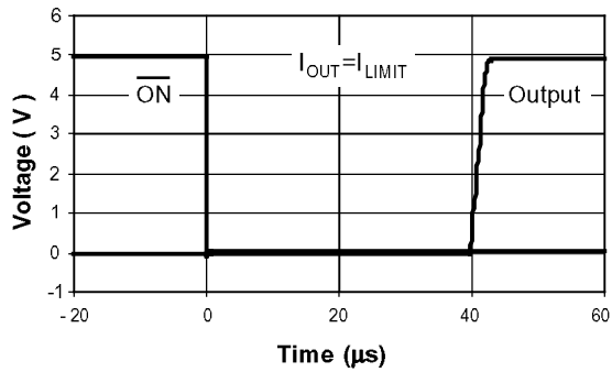
Turn-On R_L = 10\Omega , C_L = 0.47\mu F
