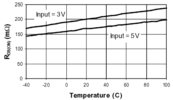
R_{DS(ON)} vs. Temperature
