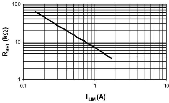
R_{SET} vs I_{LIM}
