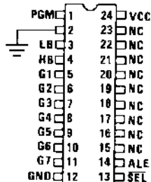
FIGURE 1. HPL-82C339 EDIT MODE PINOUT
