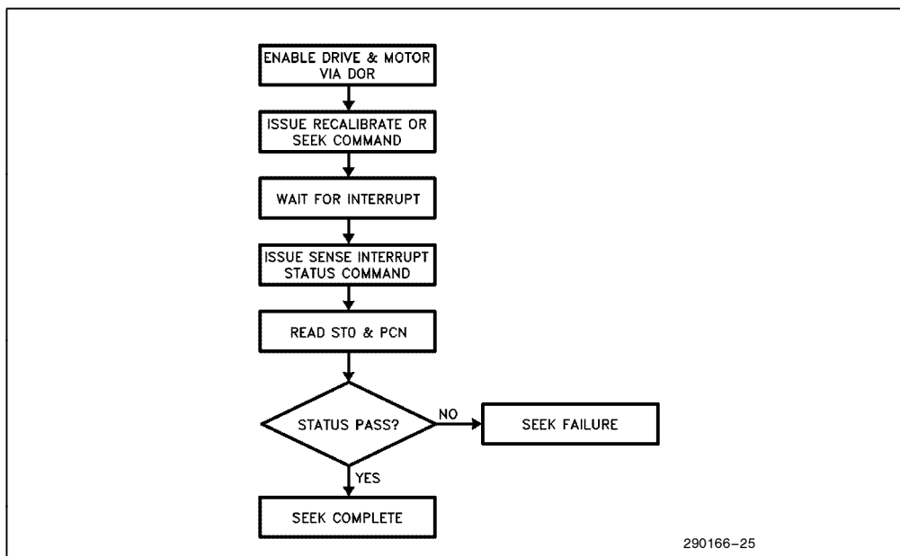
Figure 8-4. Recalibrate and Seek Operations
