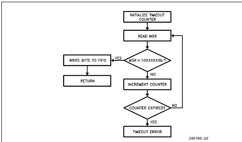
Figure 8-1. Send_Byte Routine
