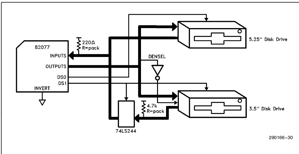
Figure 9-4. Combined 3.5" and 5.25" Drive Interface
