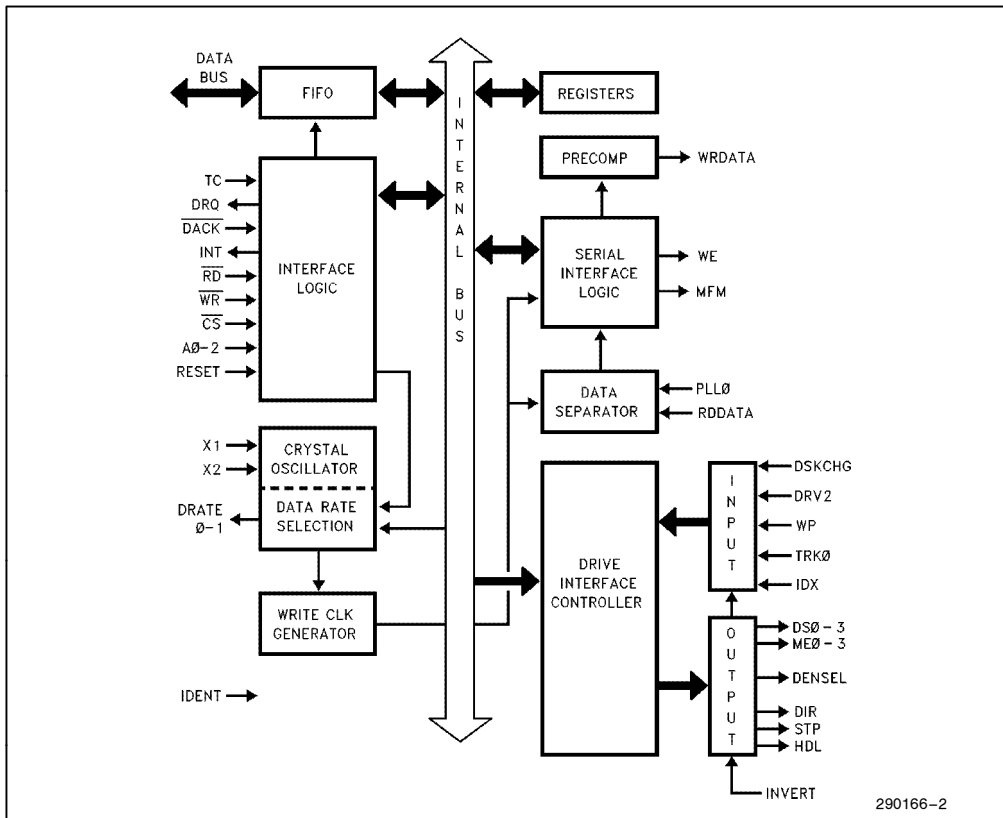
Figure 1-1. 82077AA Block Diagram
