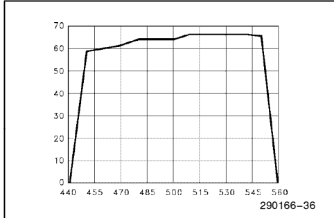
Figure 13-1. Typical Jitter Tolerance vs Data Rate (Capture Range) (±0% ISV, 500 Kbps)
