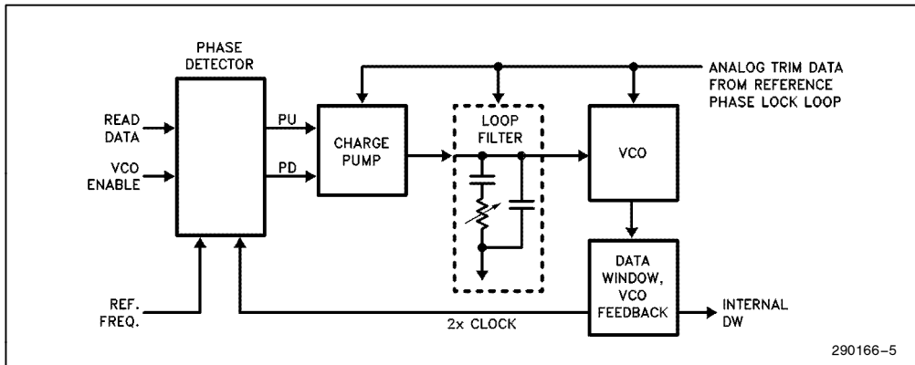
Figure 3-2. Data PLL
