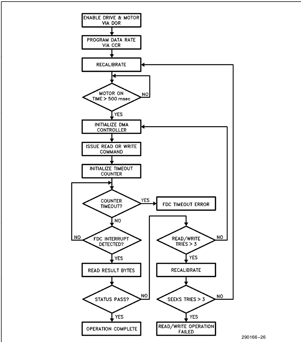
Figure 8-5. Read/Write Operation
