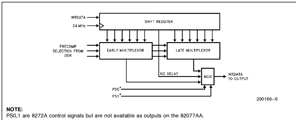
Figure 3-3. Precompensation Block Diagram
