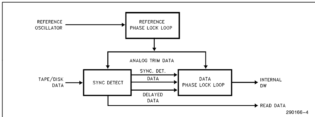
Figure 3-1. Data Separator Block Diagram
