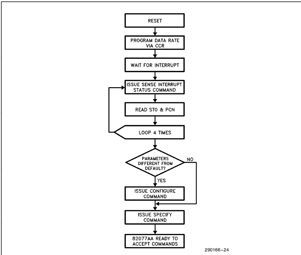
Figure 8-3. Initialization Flowchart
