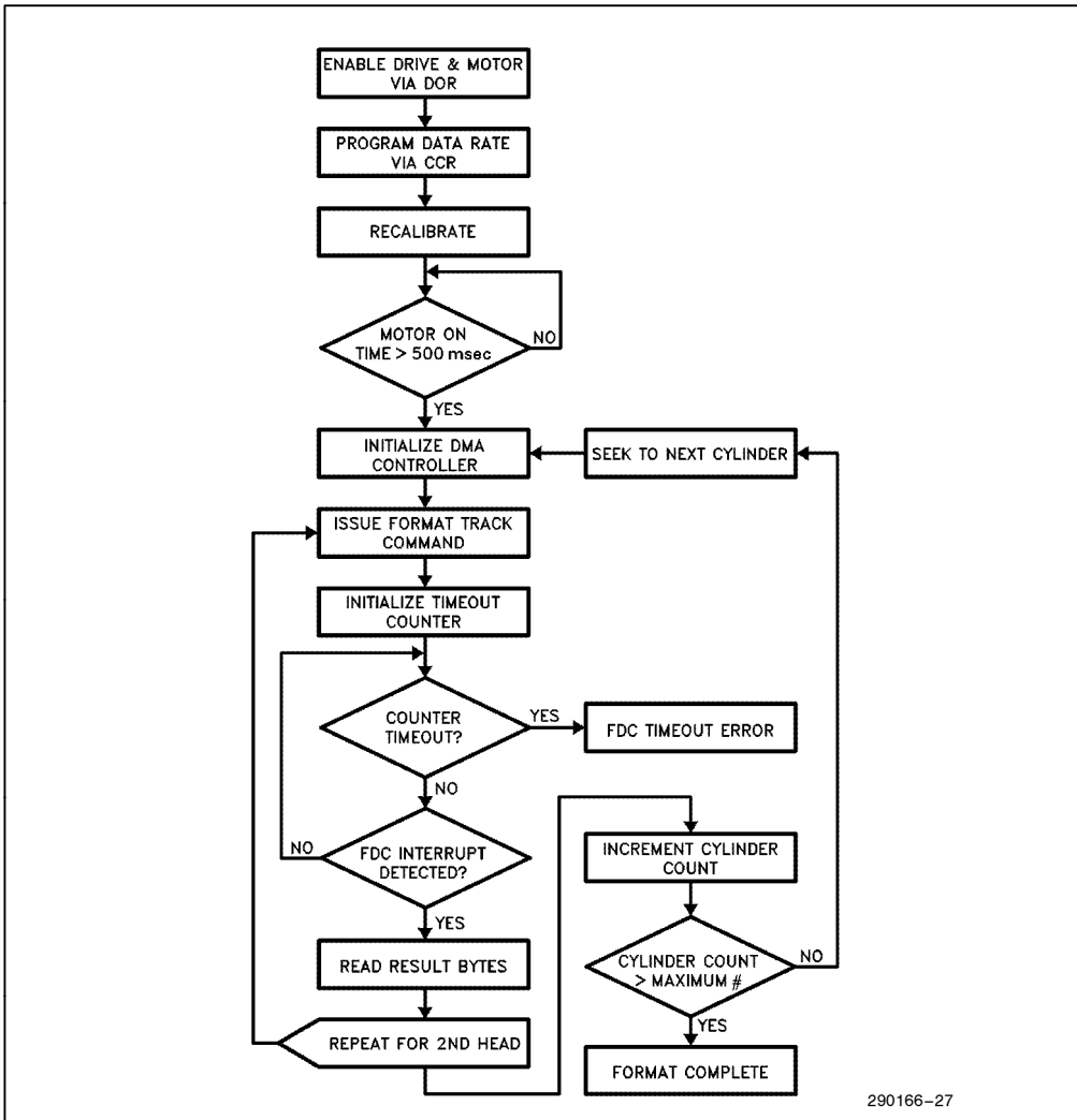
Figure 8-6 Formatting
