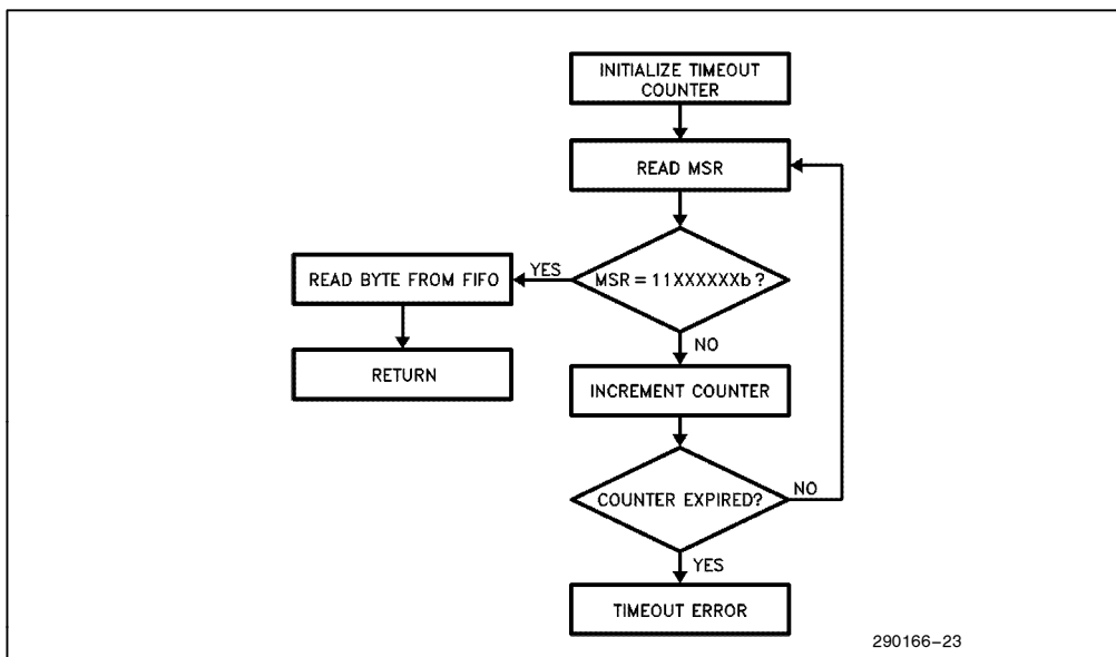
Figure 8-2. Get_byte Routine
