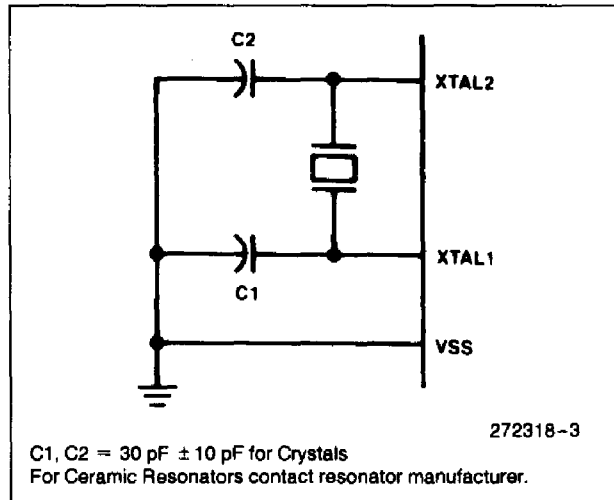
Figure 3. Oscillator Connections
