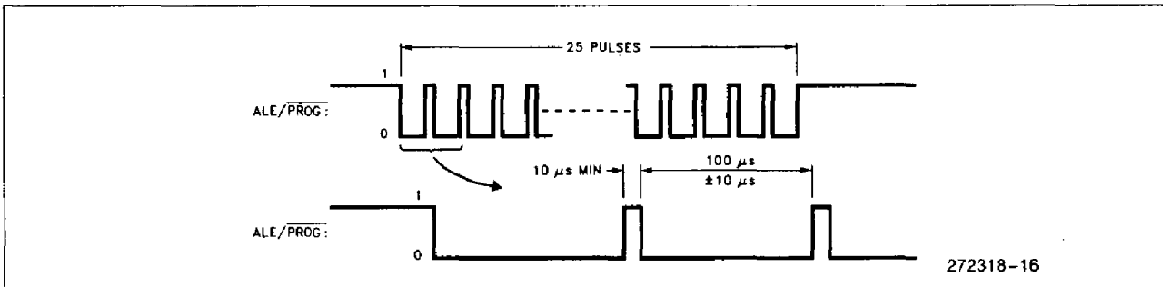
Figure 9. PROG Waveforms
