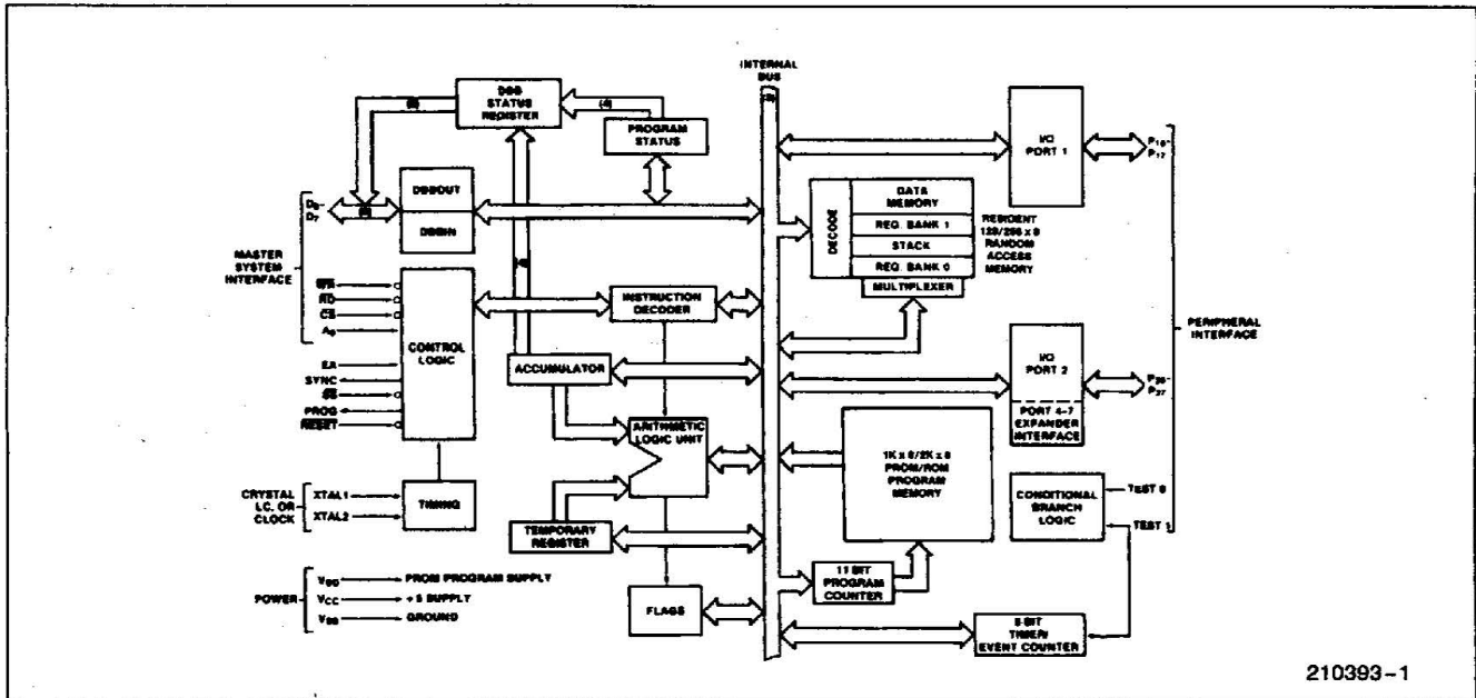
Figure 3. Block Diagram
