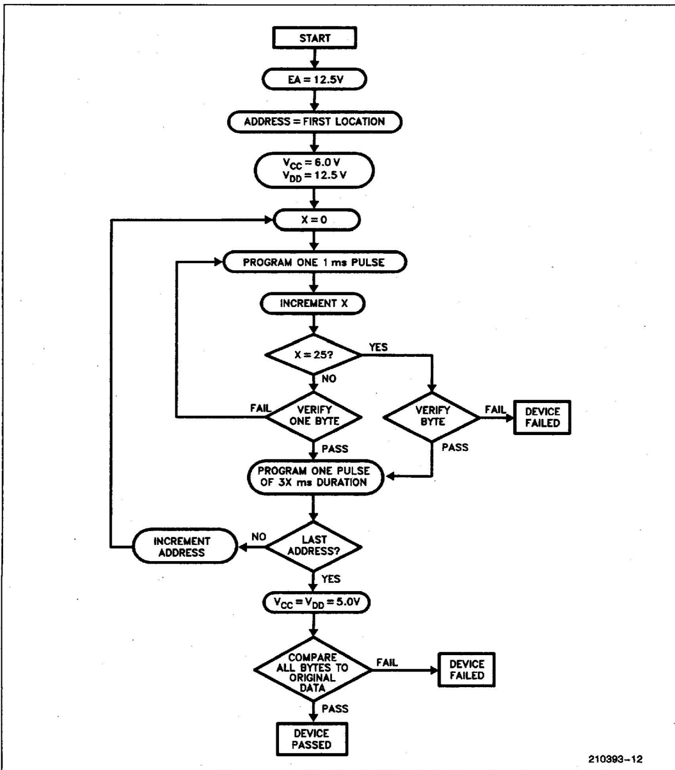
Figure 9. Programming Algorithm
