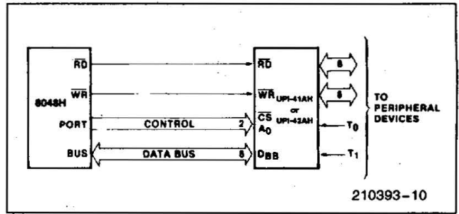
Figure 6. 8048H-UPI-41/42 Interface
