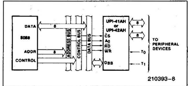
Figure 5. 8088-UPI-41AH/42AH Interface
