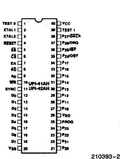
Figure 1. DIP Pin Configuration
