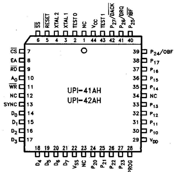
Figure 2. PLCC Pin Configuration
