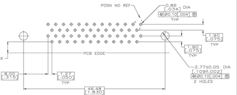
P.C. BOARD MOUNTING DIMENSIONS CONNCTOR SIDE P.C. BOARD THICKNESS 1.57±0.20 [.062±.008] PC BOARD PATTERN S
