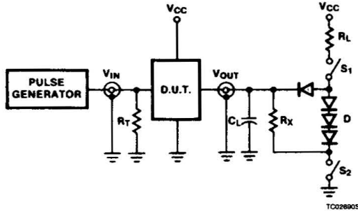
Test Circuit For 3-State Outputs
