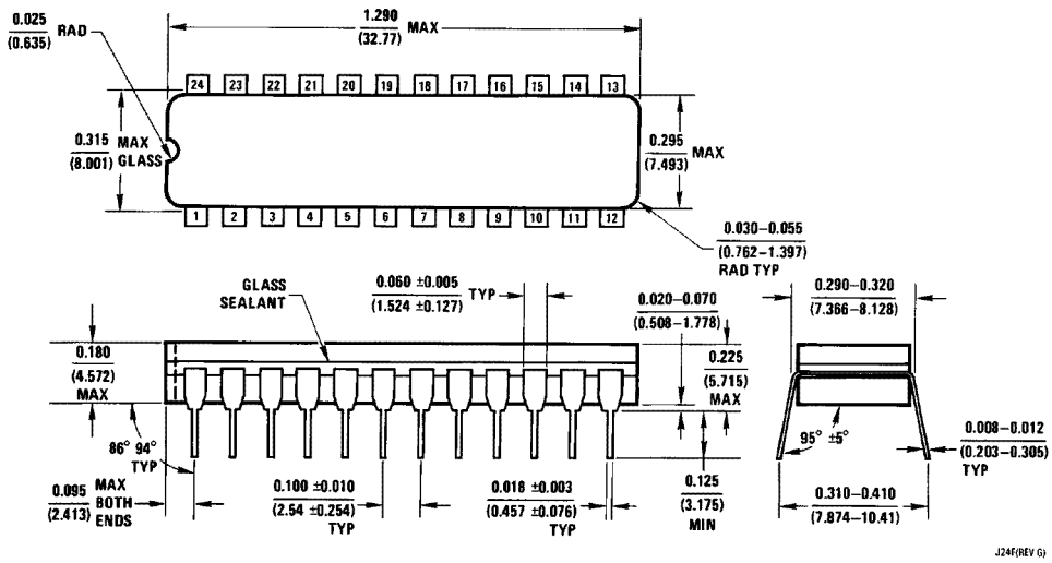
24-Lead (0.300" Wide) Ceramic Dual-In-Line Package (SD) NS Package Number J24F
