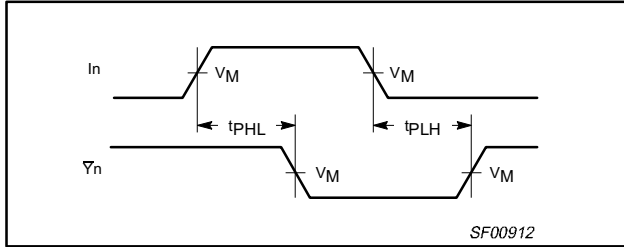
Waveform 1. For Inverting Outputs
