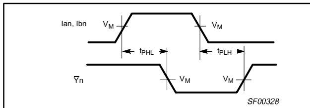
Waveform 1. Propagation delay for inverting outputs
