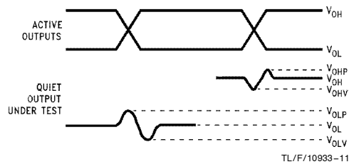
FIGURE 2. Quiet Output Noise Voltage Waveforms
