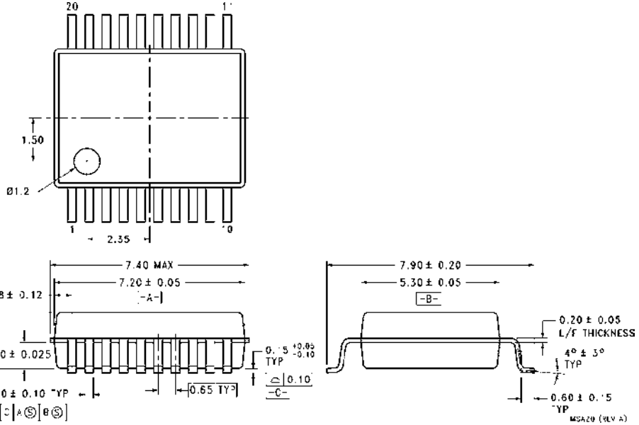
20-Lead Shrink Small Outline Package (SSOP), EIAJ TYPE II, 5.3mm Wide Package Number MSA20
