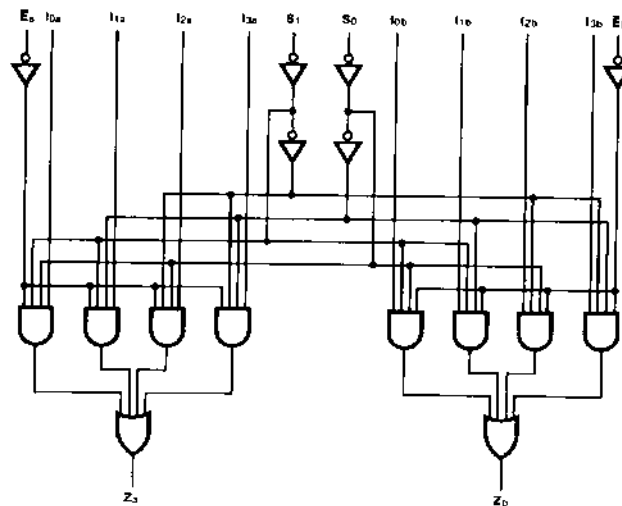
LOGIC DIAGRAM
