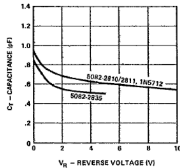
Figure 14. Typical Capacitance ( C_T ) vs. Reverse Voltage ( V_R ).
