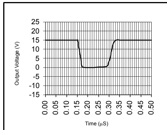
Graph 6: Output Waveform
