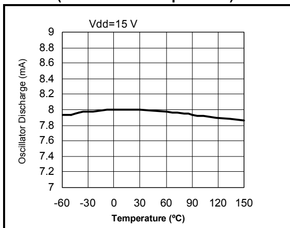
Graph 5: Oscillator Discharge (Current vs. Temperature)
