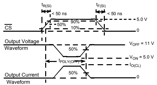
Figure 10. Turn-On/Off Waveforms
