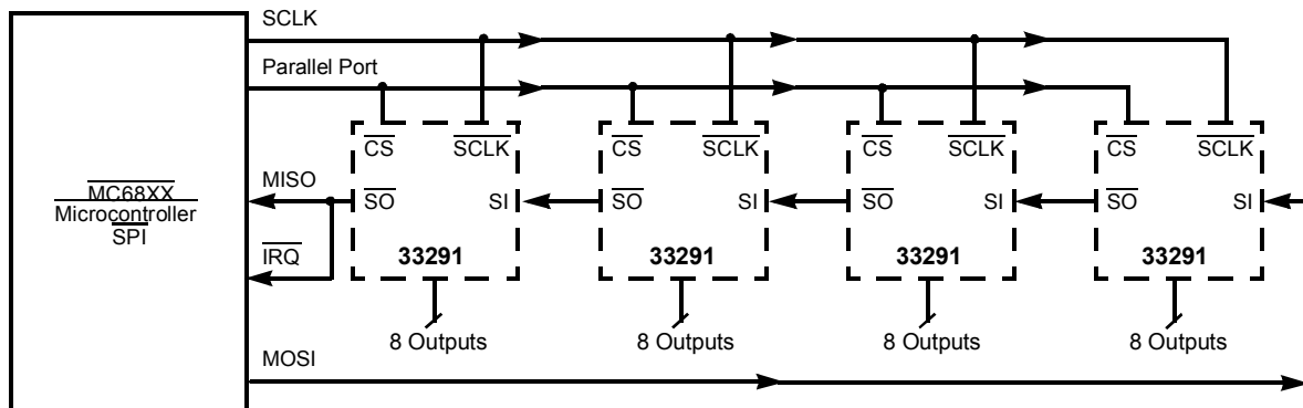
Figure 13. 33291L SPI System Daisy Chain
