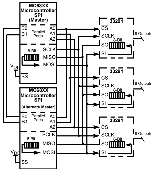
Figure 15. Multiple MCU SPI Control
