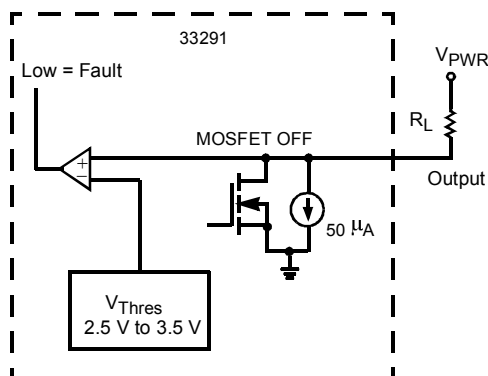
Figure 18. Output OFF Open Load Fault
