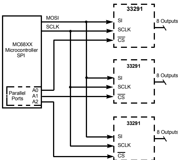
Figure 14. Parallel Input SPI Control
