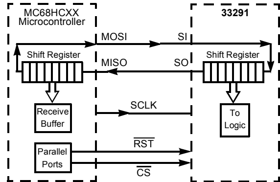
Figure 12. SPI Interface with Microcontroller
