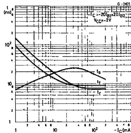
Switching Characteristics.
