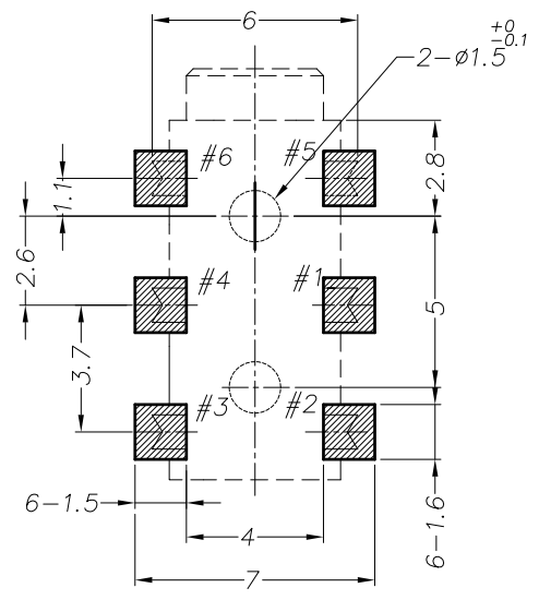
Recommended Pad Layout TOP VIEW (TOLERANCE: ±0.05)
