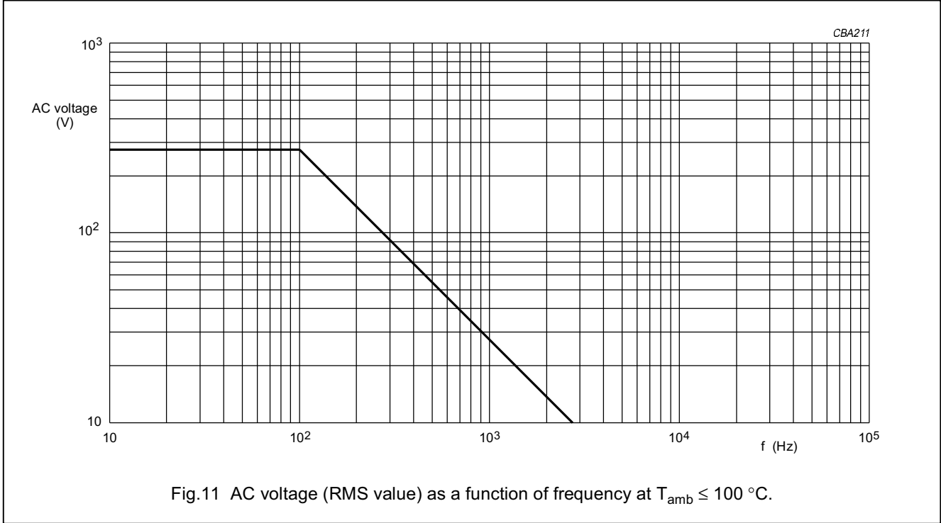
Maximum RMS voltage and AC current (sinewave) as a function of frequency for T_{amb} \leq 100\text{ }^{\circ}\text{C}
