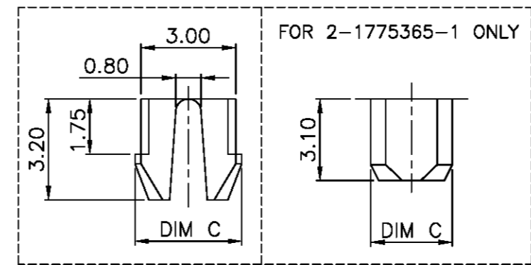
DETAIL X
