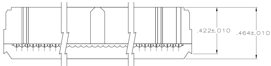
TERMINATED VIEW
