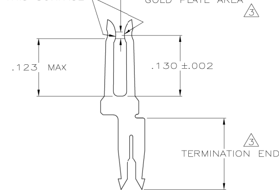
DETAIL Z SCALE 10:1 TYPICAL
