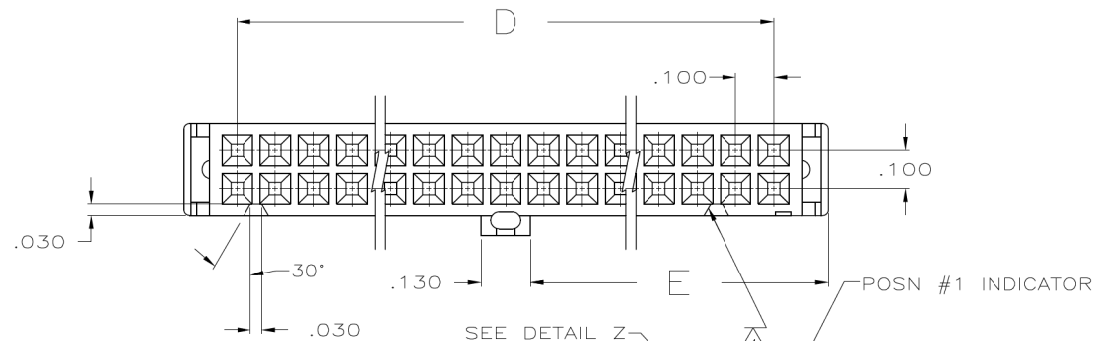
TERMINATED VIEW
