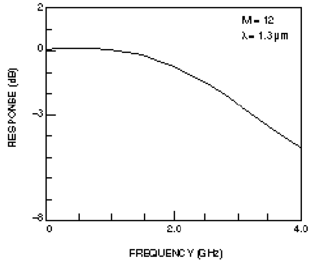
Figure 3. Frequency Response (127C)
