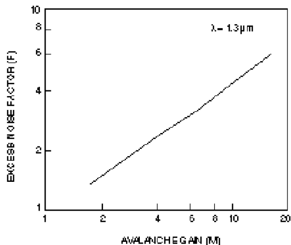
Figure 7. Excess Noise Factor vs. Gain
