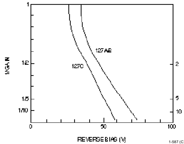
Figure 4. 1/Gain vs. Reverse Bias
