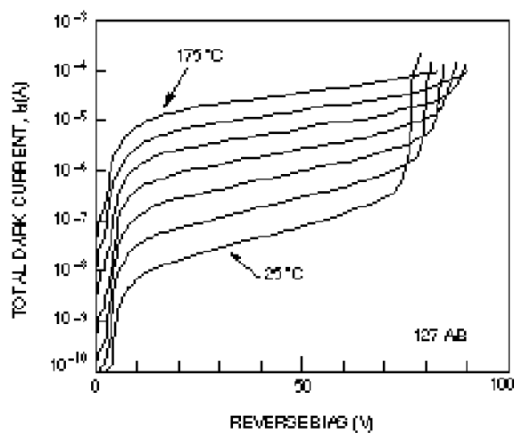
Figure 8. Dark Current vs. Voltage as a Function of Temperature at 25^\circ\text{C} Increments
