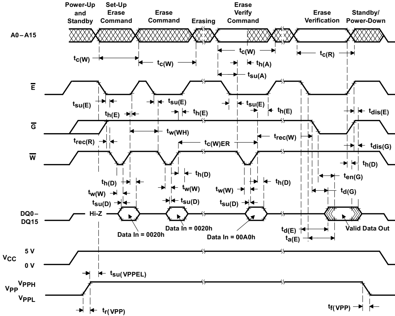
Figure 8. Flash-Erase-Cycle Timing
