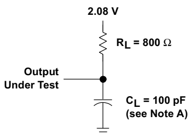
LOAD CIRCUIT
