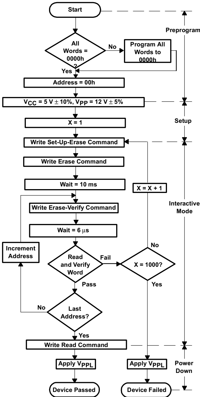
Figure 2. Flash-Erase Flowchart: Fasterase Algorithm
