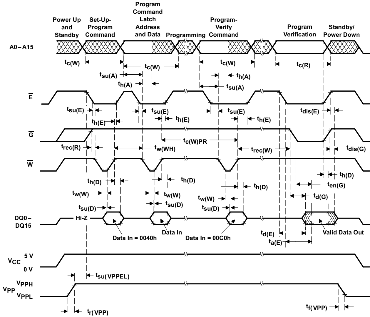
Figure 6. Write-Cycle Timing
