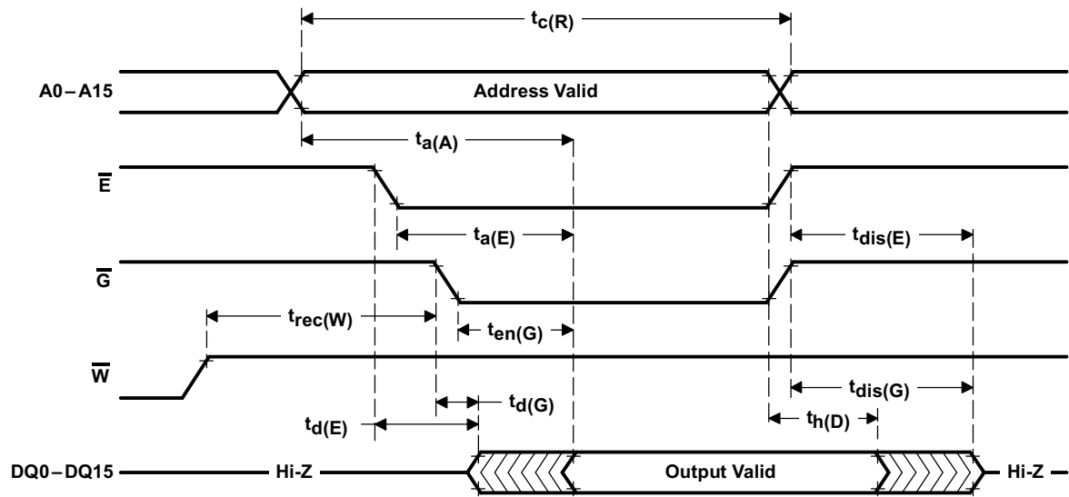
Figure 5. Read-Cycle Timing
