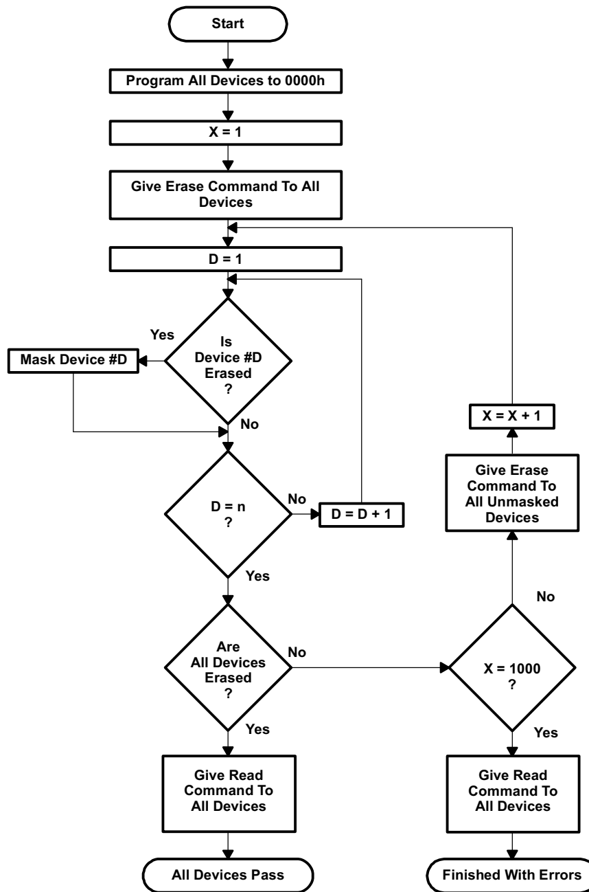
Figure 3. Parallel-Erase Flow Diagram
