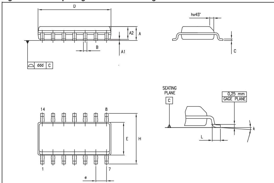
Figure 29. SO-14 package mechanical drawing
