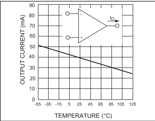
Figure 5. Current limiting
