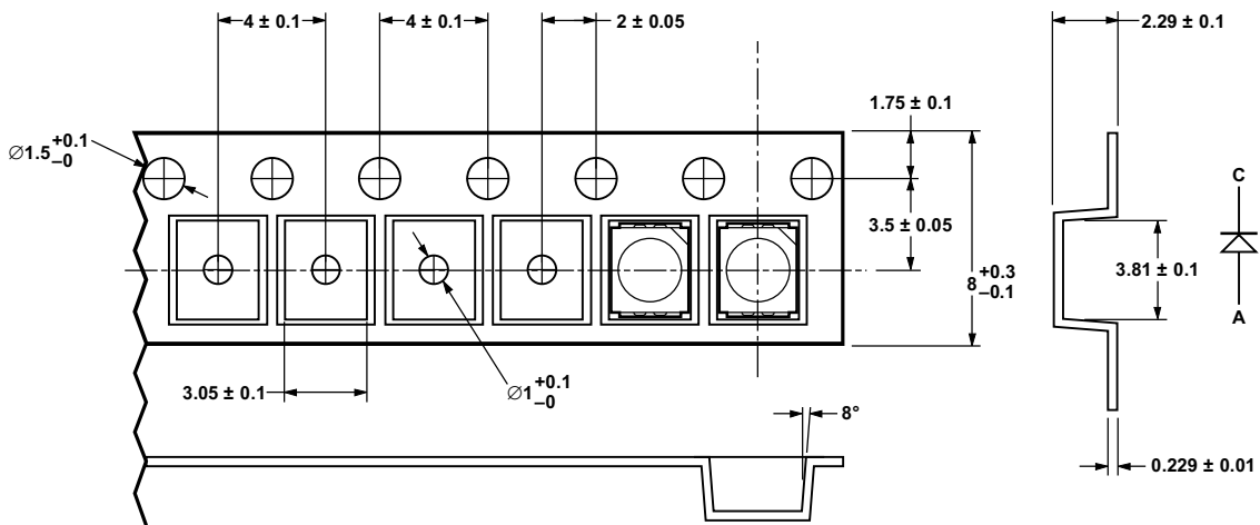
Figure 10. Tape dimension.
