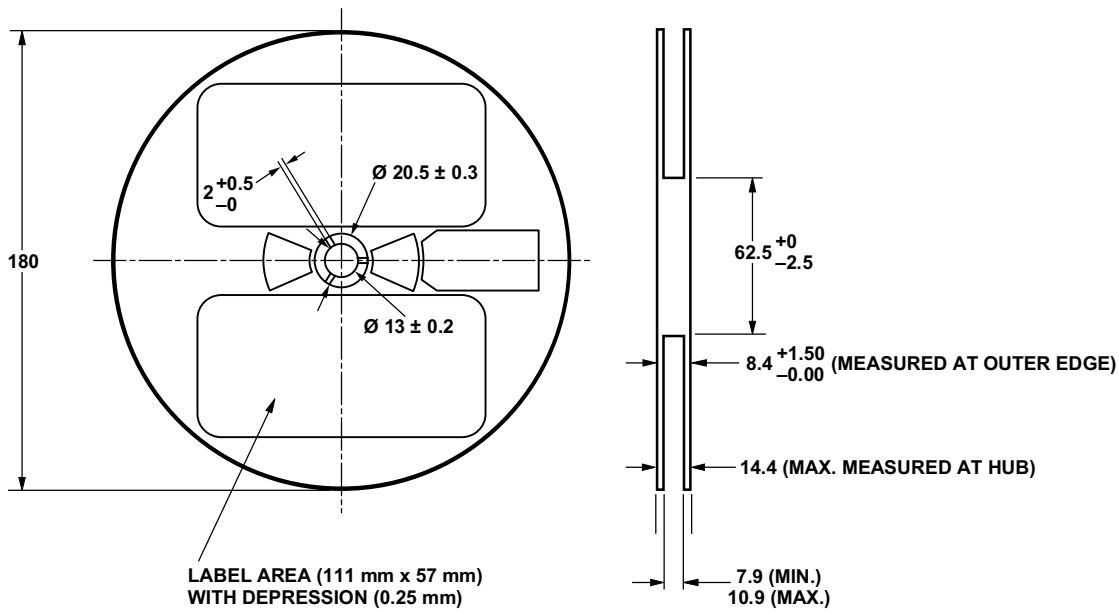
Figure 11. Reel dimension.
