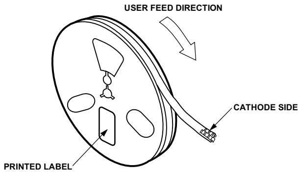
Figure 12. Reeling orientation.
