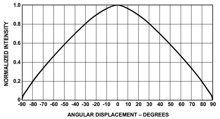
Figure 6. Radiation Pattern.
