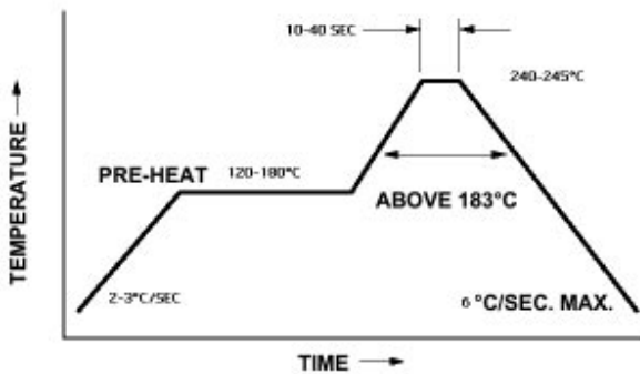
Figure 7a. Recommended wave soldering profile.
