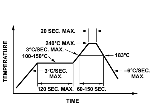
Figure 7. Recommended reflow soldering profile.
