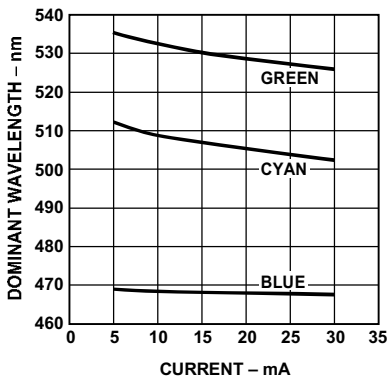
Figure 5. Dominant wavelength vs. forward current – InGaN devices.
