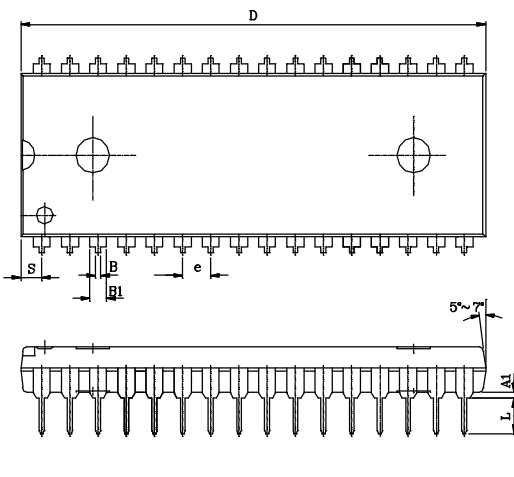
PDIP - 32
